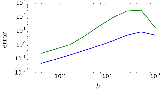
Figure 4: Error for solving the heat equation at various time steps using the projected implicit Euler method (blue), and the projected trapezoidal method (green).
