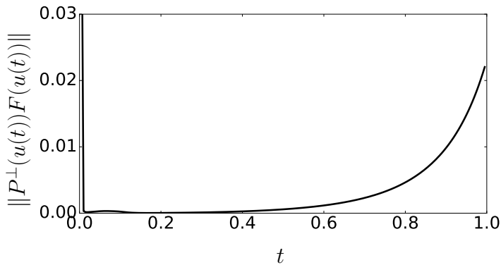
Figure 1: Component in the normal space of the right-hand side of (10), plotted against time. \|F(u(t))\| ranges between 3.2 and 9.0 over the same time interval, and the norm of the non-linear term ranges between 0.62 and 4.2. The spike near t = 0 is due to the initial data being rank-deficient.
