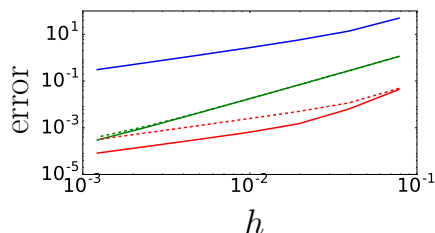
Figure 3: Error after time-stepping with standard (solid lines) and simplified (dashed) explicit Runge–Kutta methods of first, second and third order, for the same non-linear lattice Schrödinger equation as before, with \alpha = 0.1 .
