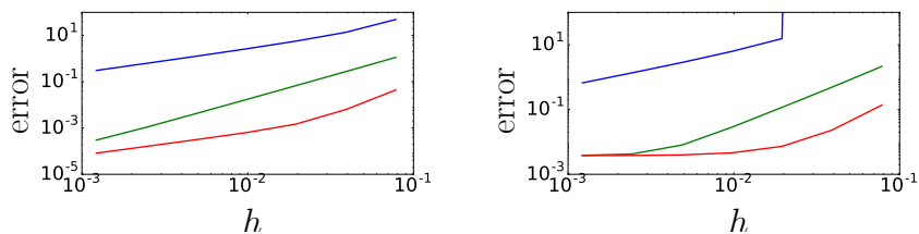
Figure 2: Error after time-stepping with PRK1 (blue), PRK2 (green), and PRK3 (red). \alpha = 0.1 (left) and \alpha = 0.3 (right).
